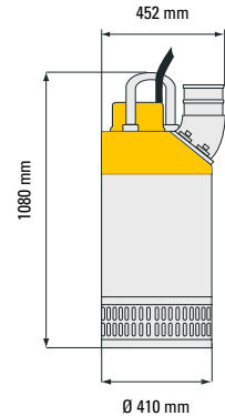
Dimensions (mm)
